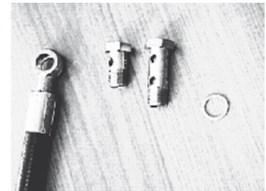
Banjo fitting, bolt, double bolt, copper ring
